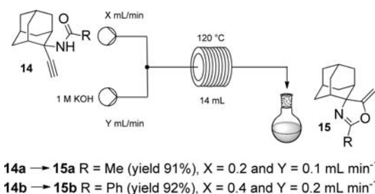
Figure 12. Flow schemes for the 5-enol-exodig cyclisation of compounds 14 to oxazolines 15.
