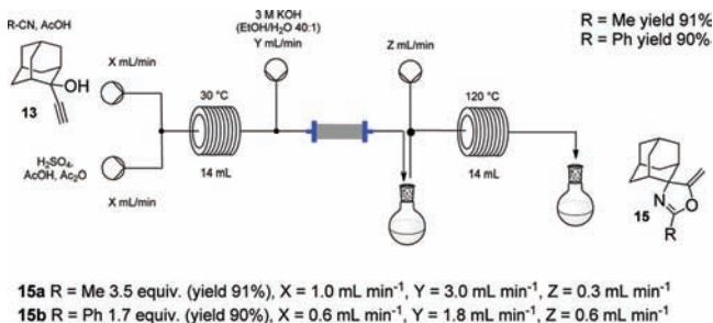
Figure 13. Combined Ritter reaction and 5-enol-exodig cyclisation to oxazolines 15.
